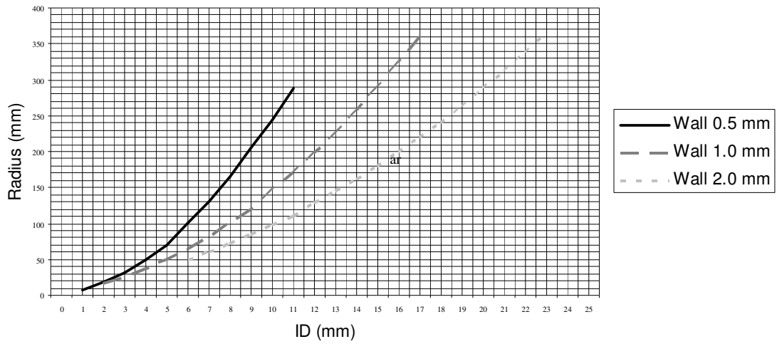
Bending radius for FEP at 25° C
